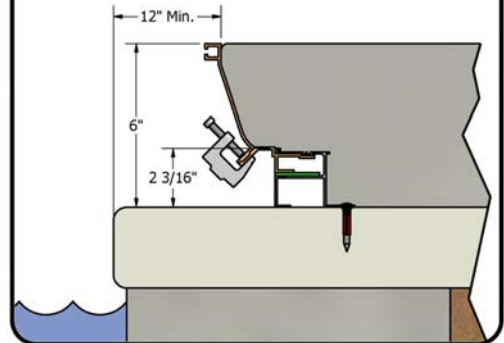
Raised Deck on Deck Retainer (55049) w/ 2-Piece Angle Coping Form (55062) - Form Kit: PCS 2121 -
